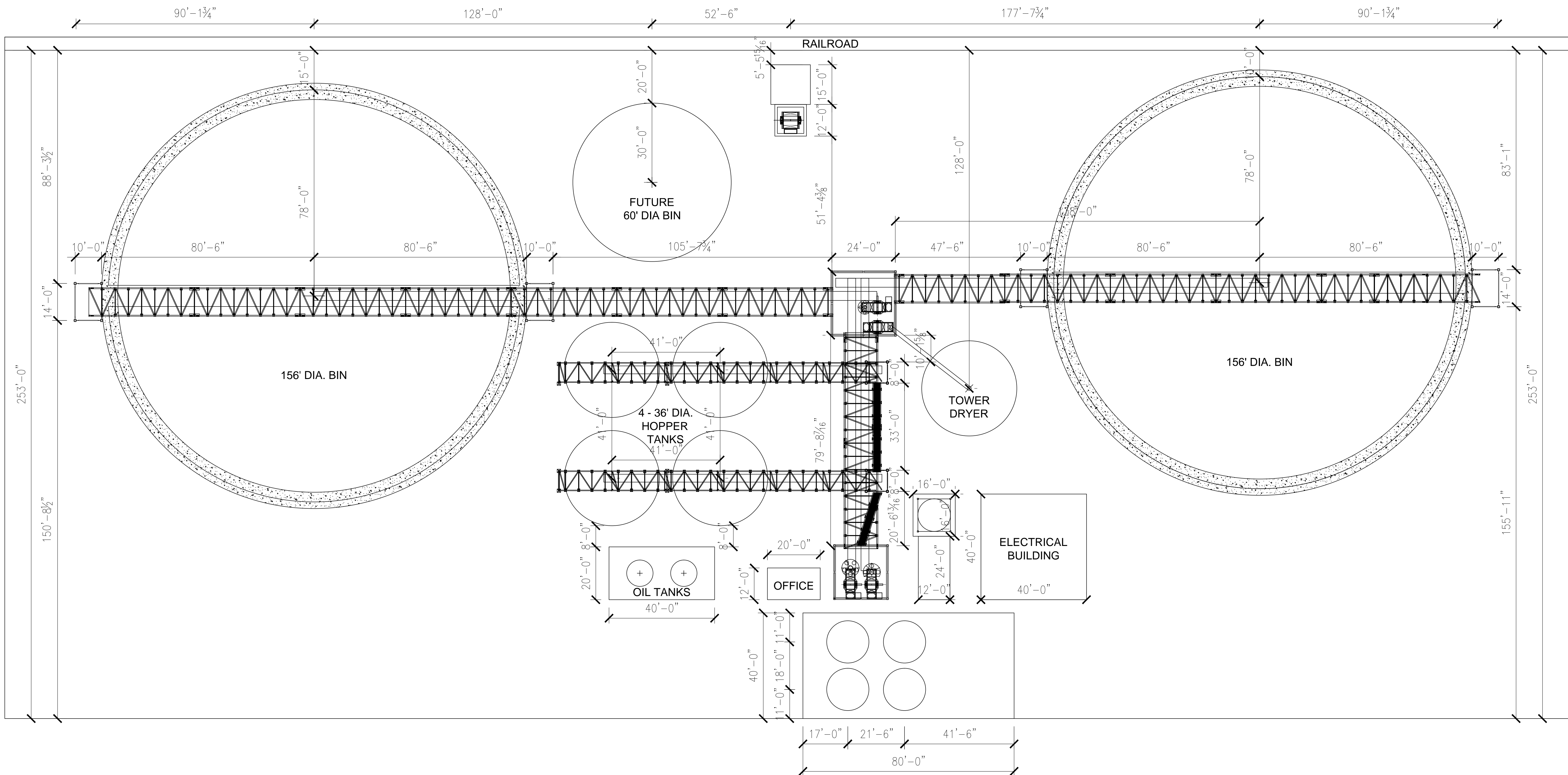
TOP PLAN VIEW
